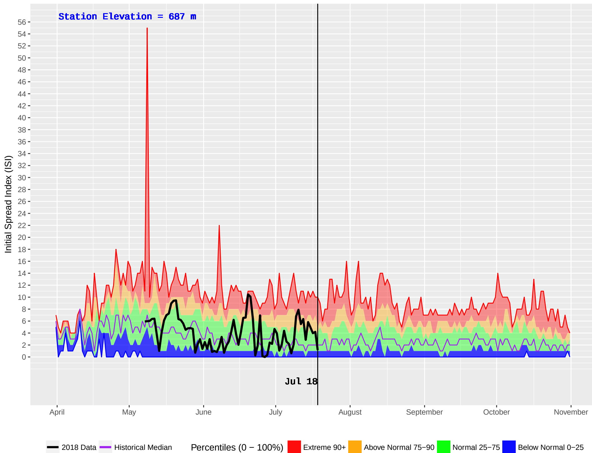
KETCHIKA (444) : Historical (1986–2016) and Current (2018) Daily Initial Spread Index (ISI)
