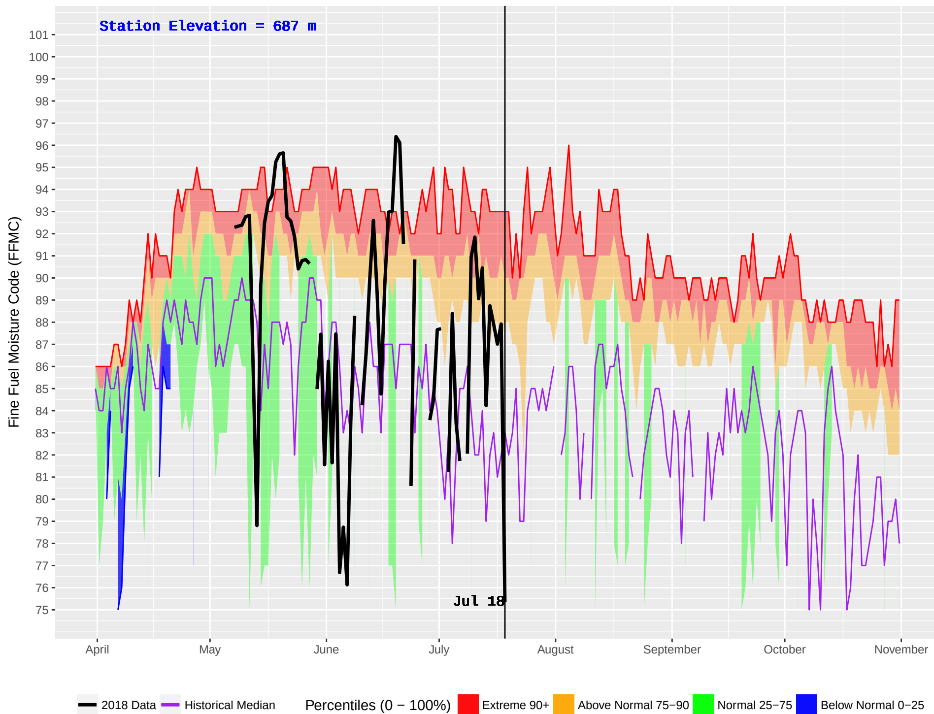
KETCHIKA (444) : Historical (1986–2016) and Current (2018) Daily Fine Fuel Moisture Code (FFMC)
