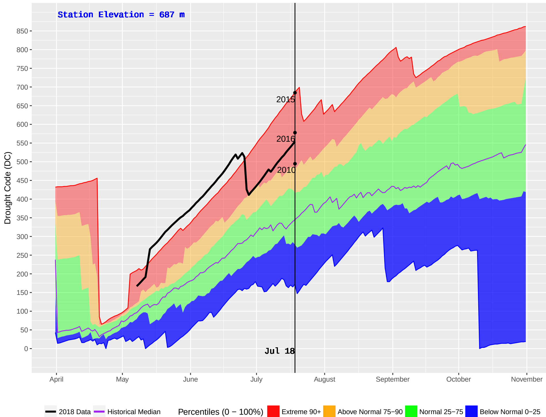
KETCHIKA (444) : Historical (1986–2016) and Current (2018) Daily Drought Code (DC)
