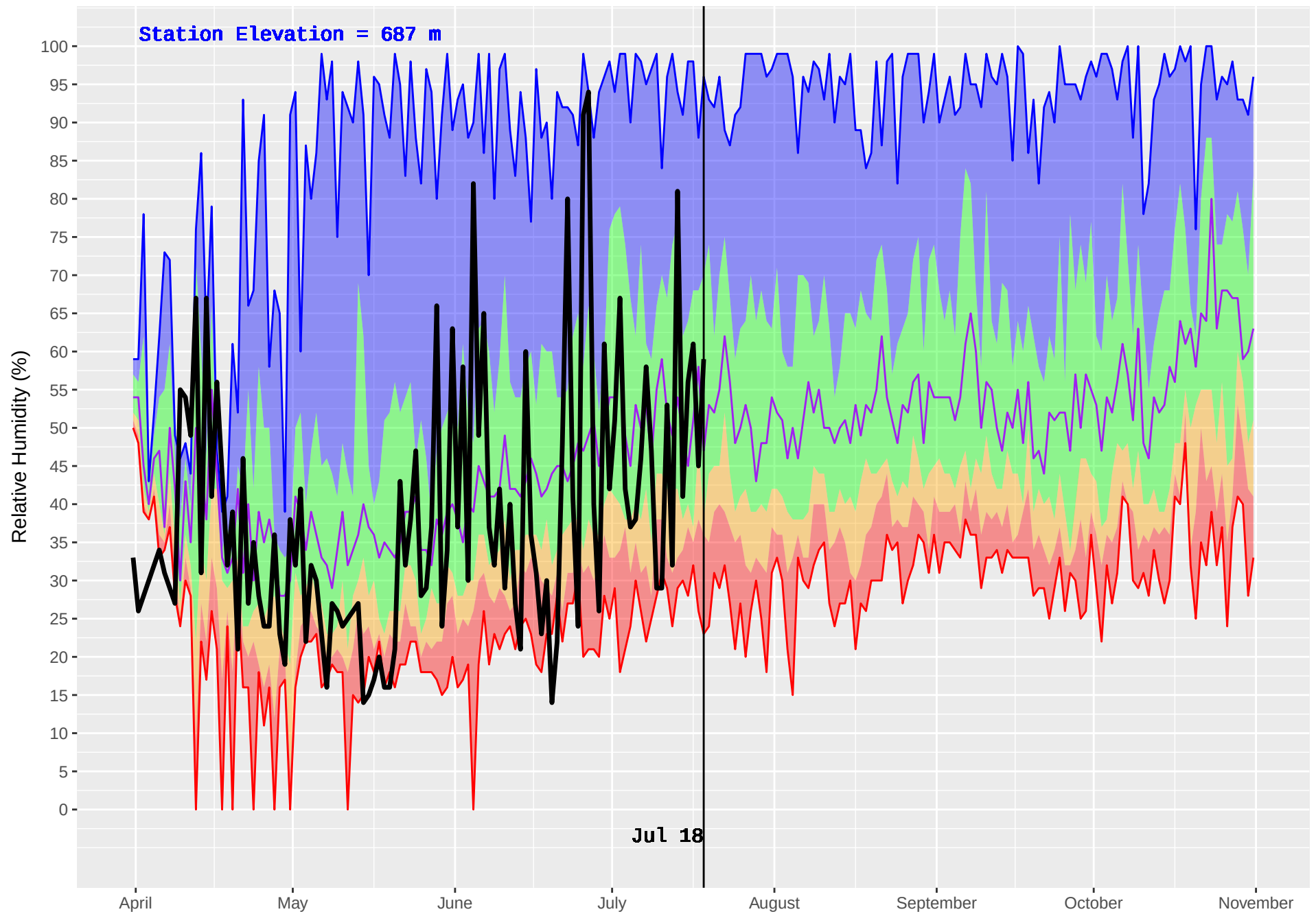
KETCHIKA (444) : Historical (1986–2016) and Current (2018) Daily Relative Humidity
