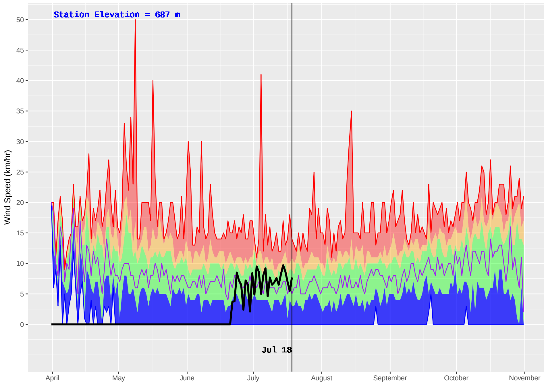
KETCHIKA (444) : Historical (1986–2016) and Current (2018) Daily Wind Speed
