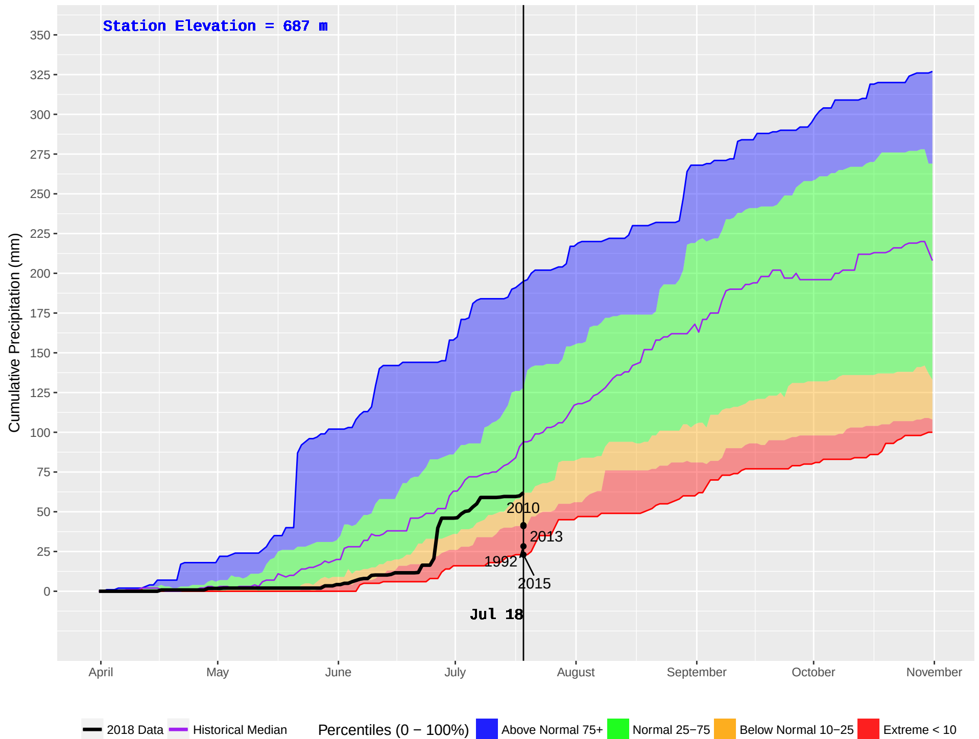
KETCHIKA (444) : Historical (1986–2016) and Current (2018) Daily Cumulative Precipitation
