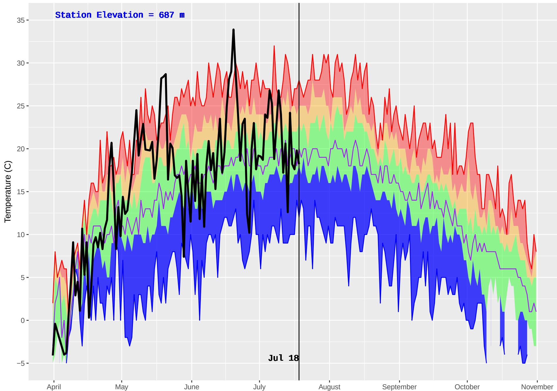
KETCHIKA (444) : Historical (1986–2016) and Current (2018) Daily Temperature
