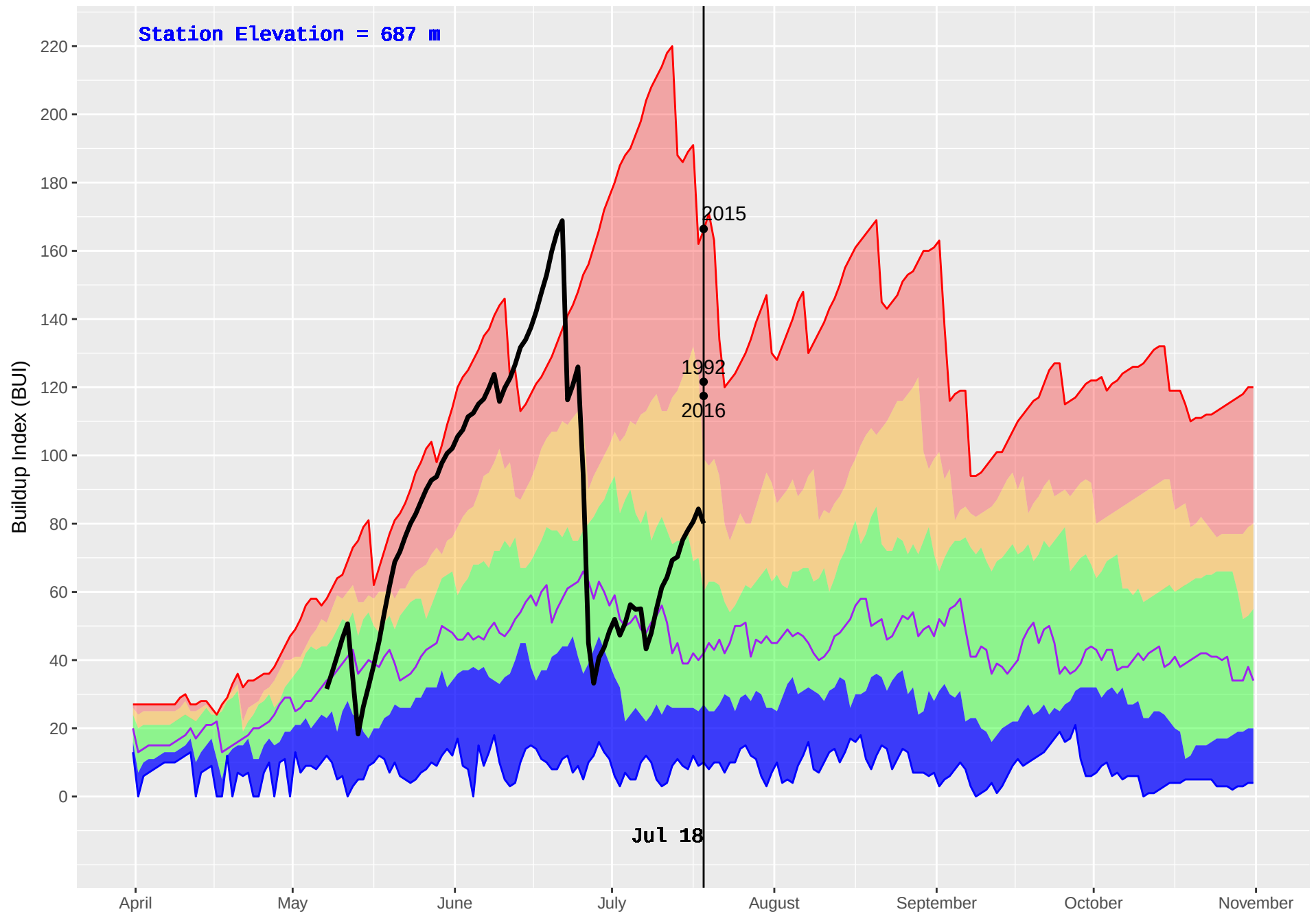
KETCHIKA (444) : Historical (1986–2016) and Current (2018) Daily Buildup Index (BUI)
